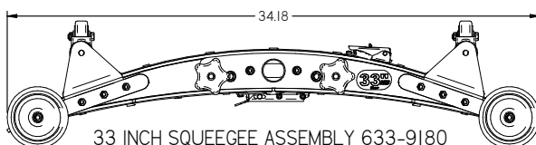
33 INCH SQUEEGEE ASSEMBLY 633-9180
